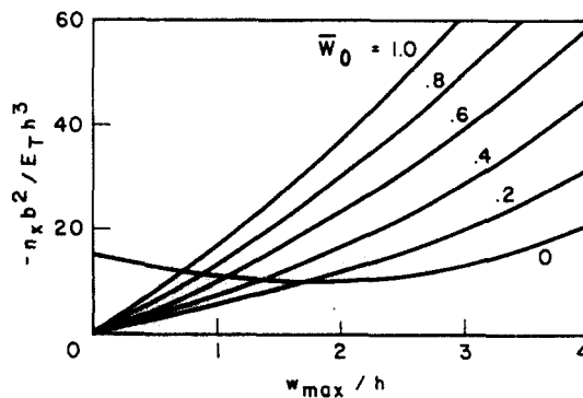
Fig. 5. Postbuckling load-deflection curves for a three-layer cross-ply glass-epoxy cylindrical panel of different initial imperfections ( a/b = 1 , K_R = 20 , \bar{W}_m = 0 for m, n > 1 ).
